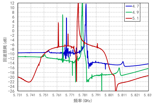
RFOUT回波损耗 VS 频率 (Vt=0.75V, Vcc=5.1V, 85°C)
